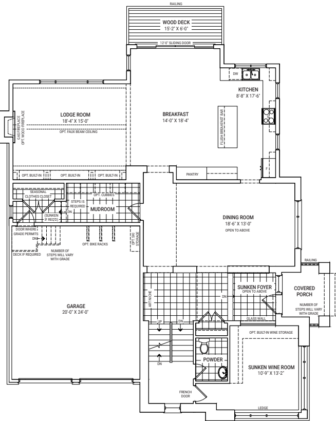
GROUND FLOOR PLAN ELEVATION A
